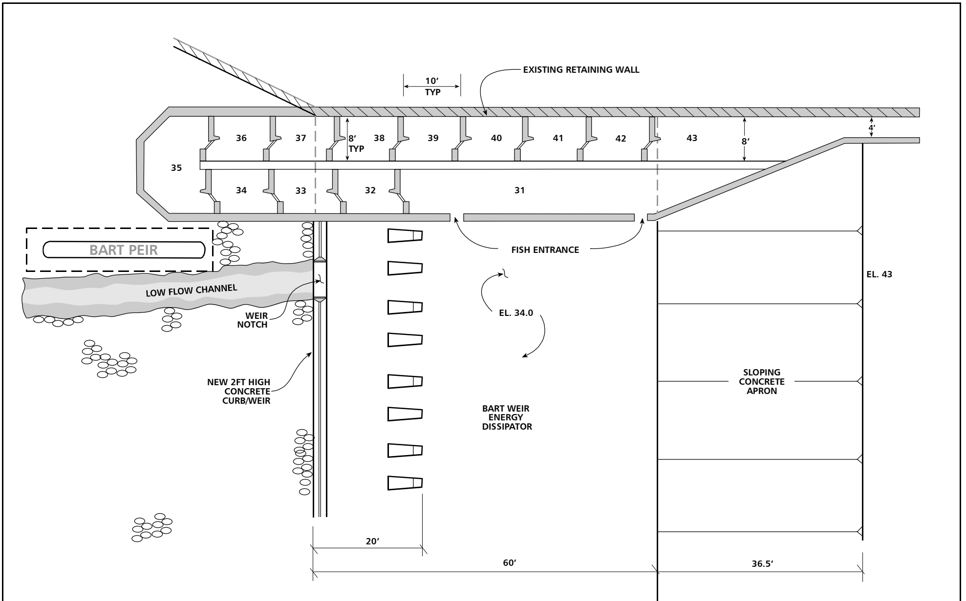
Figure 6-Detail Plan Proposed Fishway at B.A.R.T. WEIR and MIDDLE Inflatable DAM Alameda Creek Fish Passage
